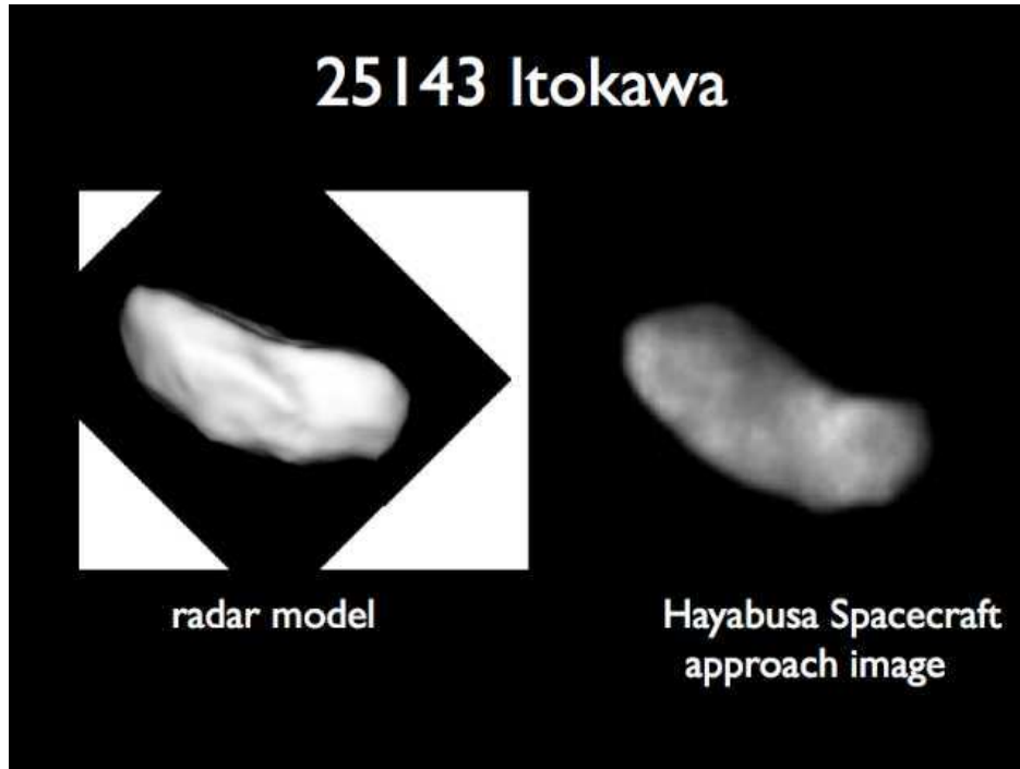
Figure 5: Comparison of Radar Model and In Situ Hayabusa Spacecraft Camera Imagery for NEA 25143 Itokawa
